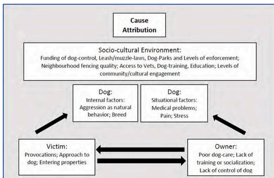
Figure 1. Cause attribution.
