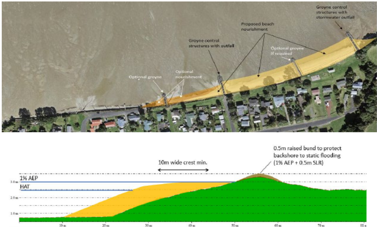
Figure 2: A typical beach cross section showing the imported sand (yellow) and raised berm (brown) relative to present day tidal levels.
